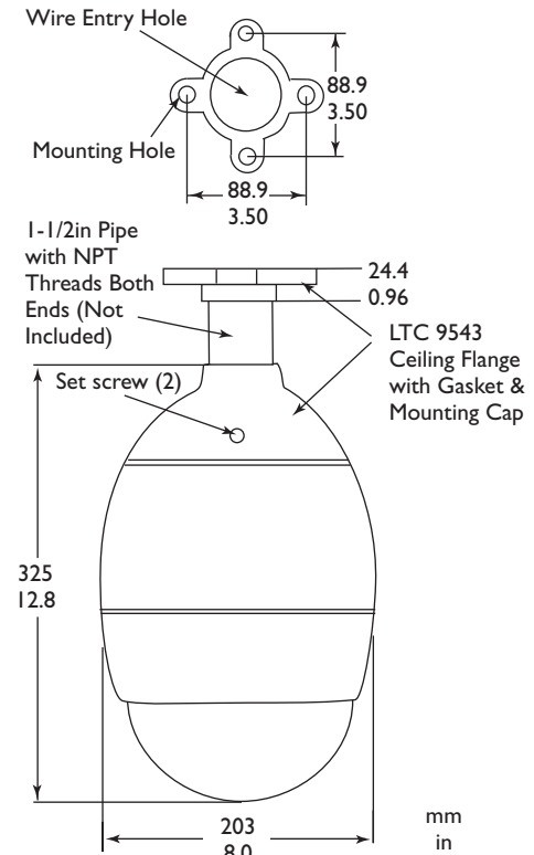
Figure 1: Ceiling/Pipe Mounting
